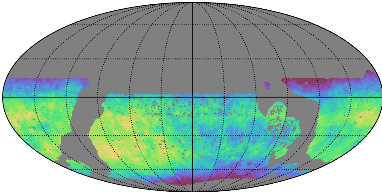
baseline_v3.2_10yrs WFD i band: Median fiveSigmaDepth
