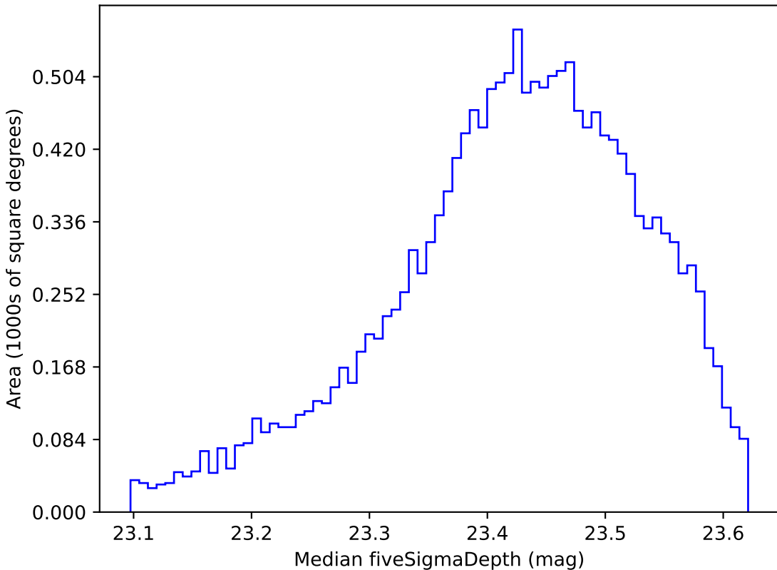
baseline_v3.2_10yrs WFD i band: Median fiveSigmaDepth
