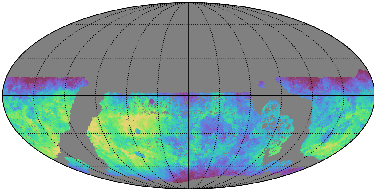
baseline_v3.2_10yrs WFD g band: Median fiveSigmaDepth
