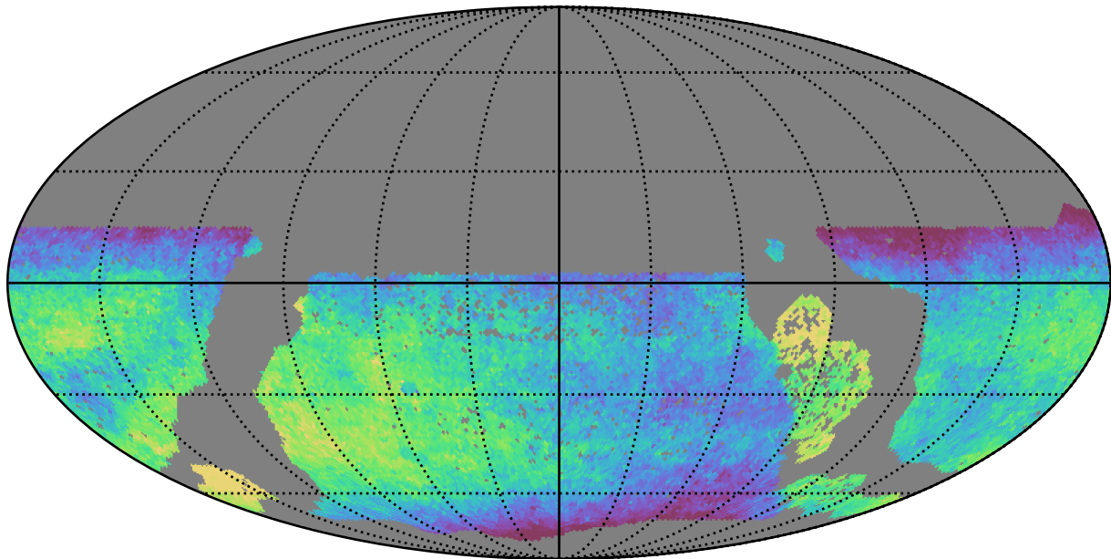
baseline_v3.2_10yrs WFD all bands: Median fiveSigmaDepth
