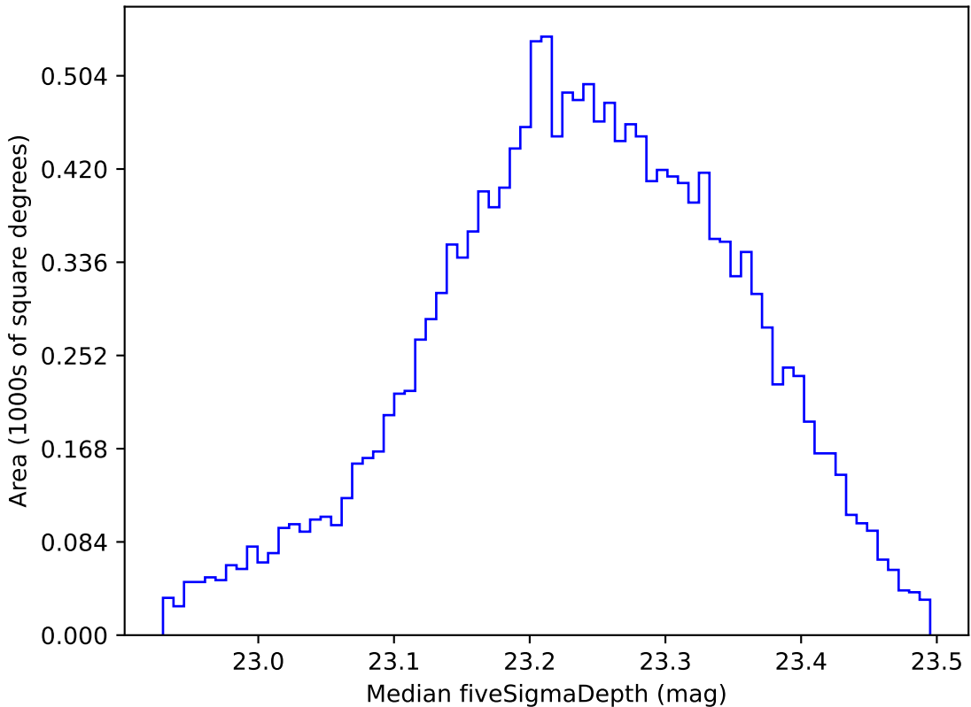
baseline_v3.2_10yrs WFD all bands: Median fiveSigmaDepth
