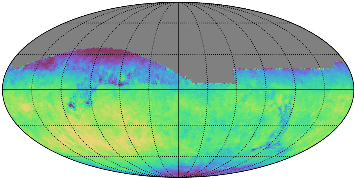
baseline_v3.2_10yrs All sky z band: Median fiveSigmaDepth
