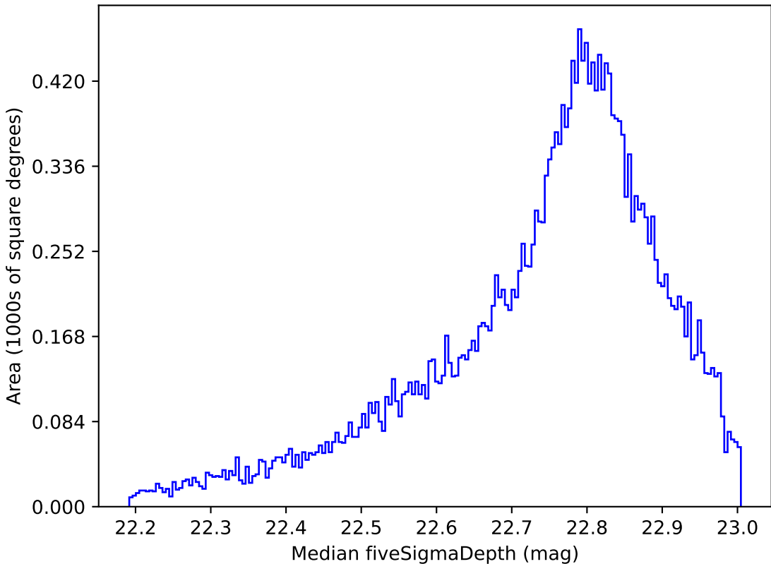
baseline_v3.2_10yrs All sky z band: Median fiveSigmaDepth
