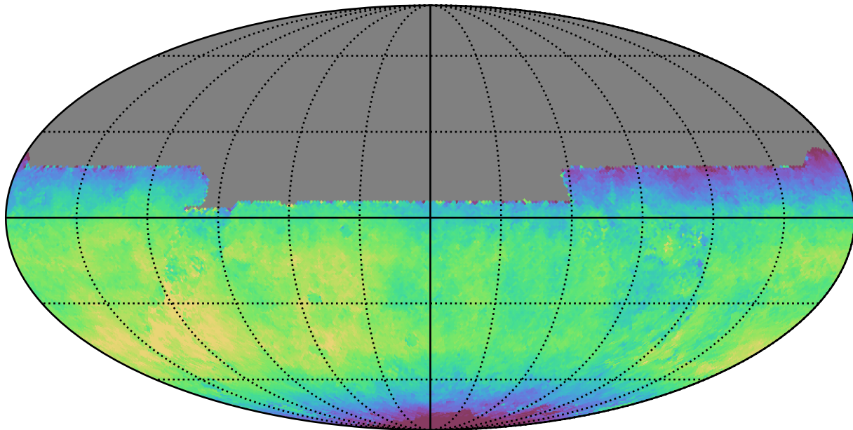
baseline_v3.2_10yrs All sky y band: Median fiveSigmaDepth
