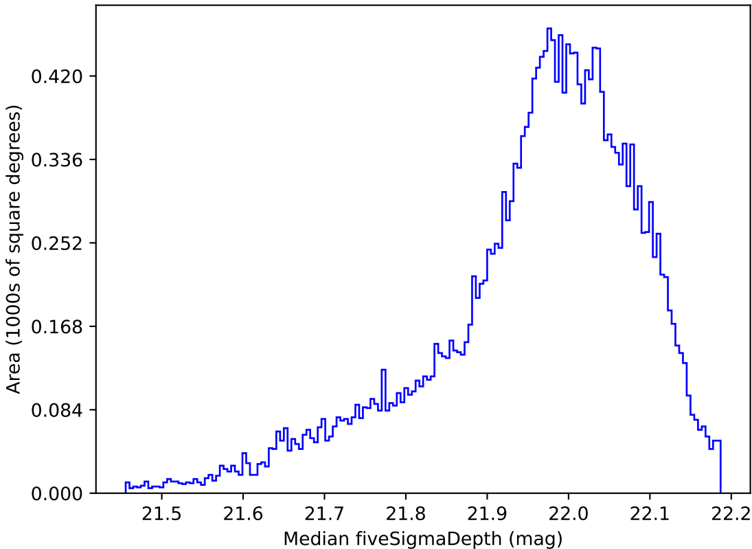
baseline_v3.2_10yrs All sky y band: Median fiveSigmaDepth
