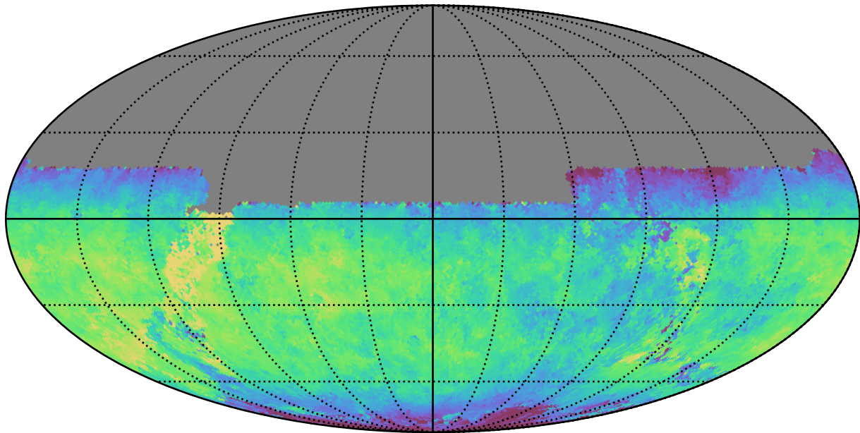
baseline_v3.2_10yrs All sky u band: Median fiveSigmaDepth
