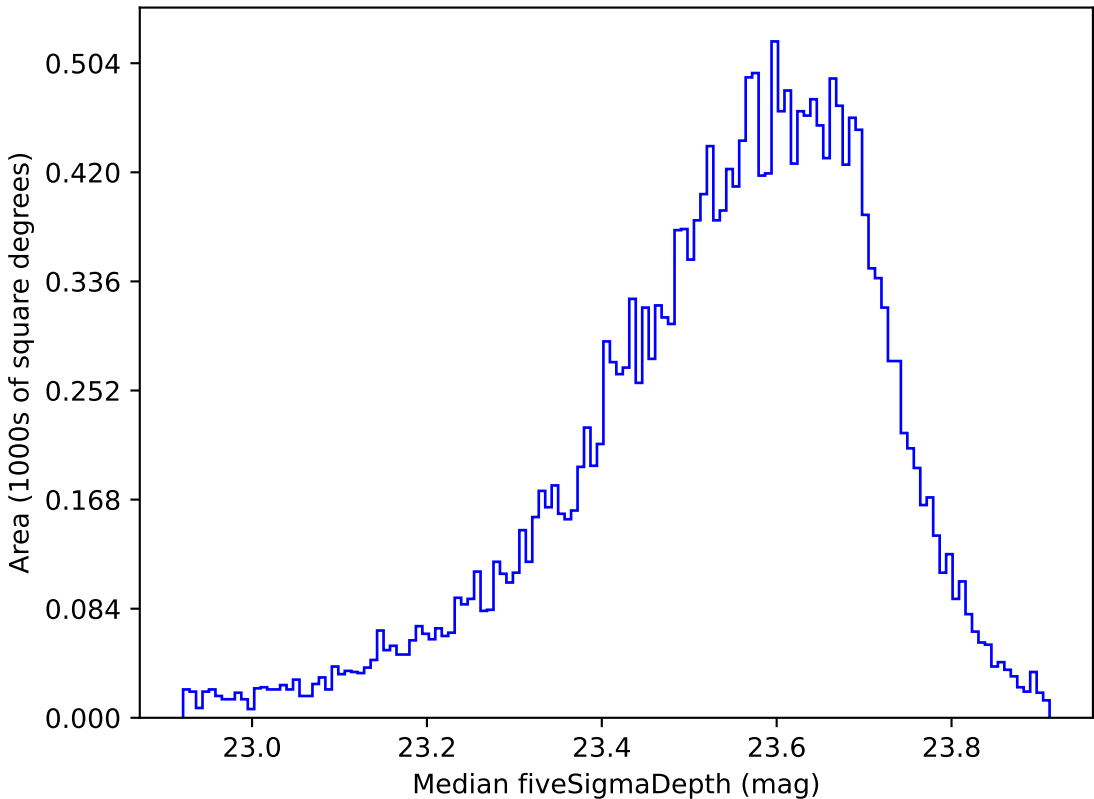
baseline_v3.2_10yrs All sky u band: Median fiveSigmaDepth
