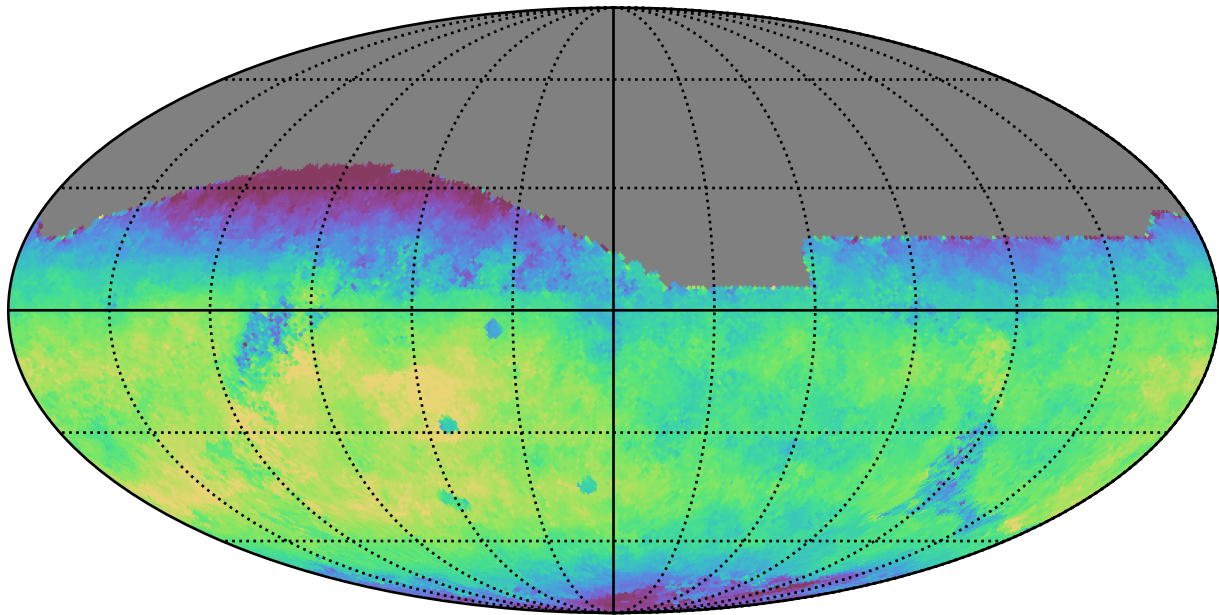
baseline_v3.2_10yrs All sky r band: Median fiveSigmaDepth
