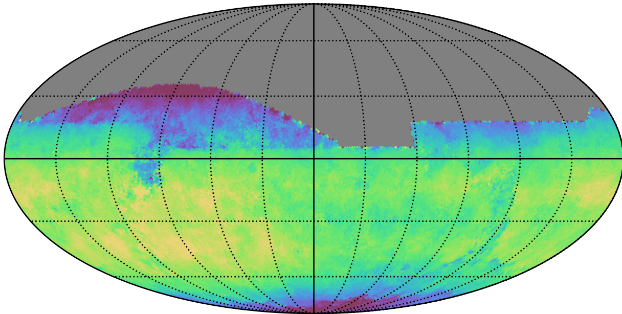
baseline_v3.2_10yrs All sky i band: Median fiveSigmaDepth
