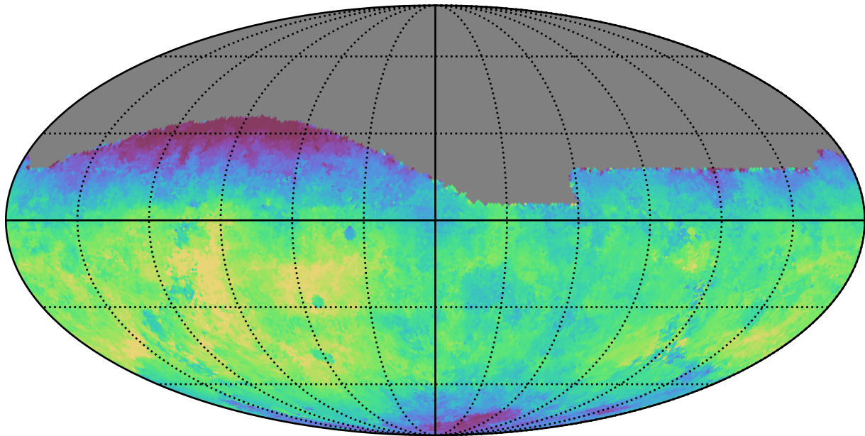
baseline_v3.2_10yrs All sky g band: Median fiveSigmaDepth
