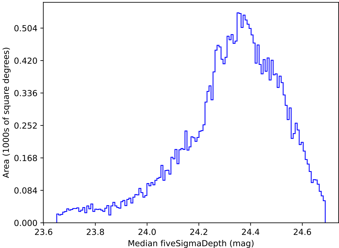
baseline_v3.2_10yrs All sky g band: Median fiveSigmaDepth
