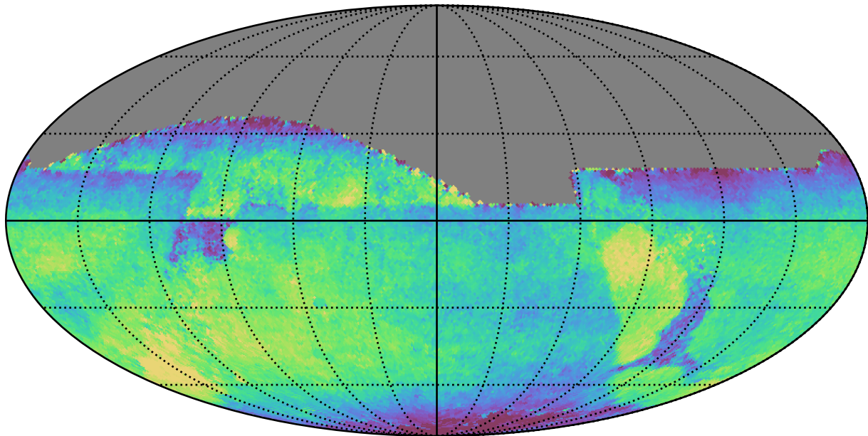
baseline_v3.2_10yrs All sky all bands: Median fiveSigmaDepth
