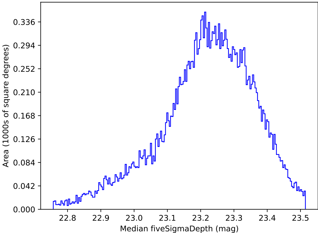
baseline_v3.2_10yrs All sky all bands: Median fiveSigmaDepth
