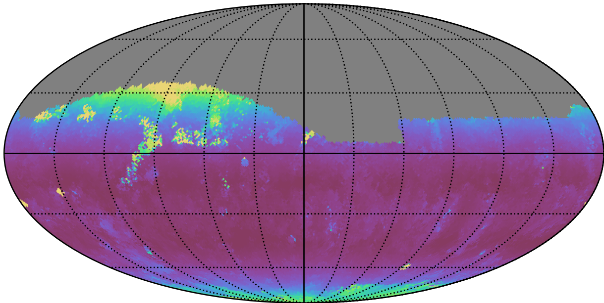
baseline_v3.2_10yrs Yr 1 z band: Median airmass
