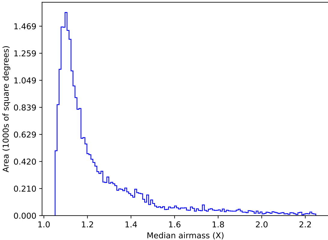
baseline_v3.2_10yrs Yr 1 z band: Median airmass
