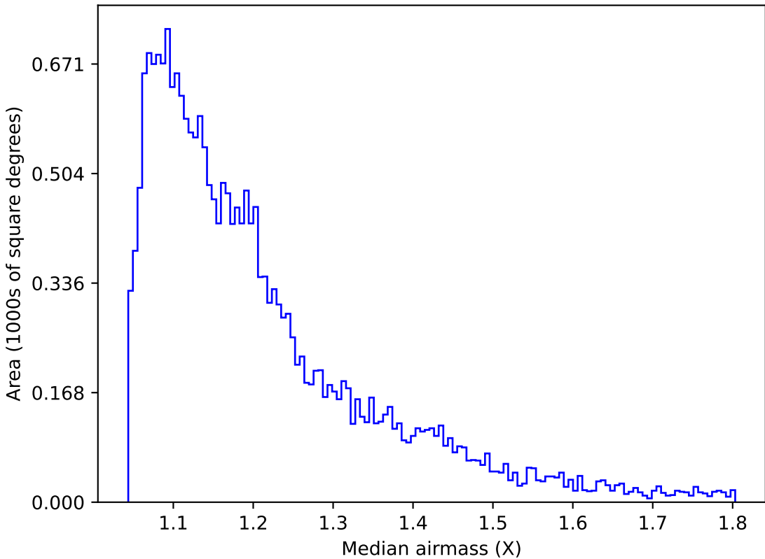
baseline_v3.2_10yrs Yr 1 u band: Median airmass
