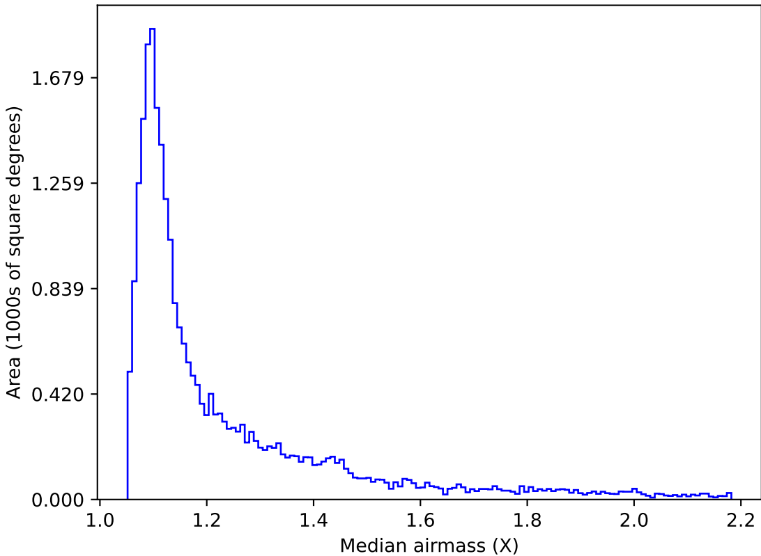
baseline_v3.2_10yrs Yr 1 i band: Median airmass
