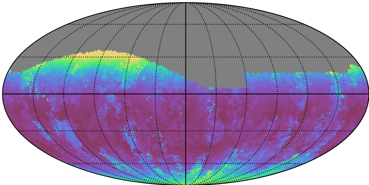
baseline_v3.2_10yrs Yr 1 g band: Median airmass
