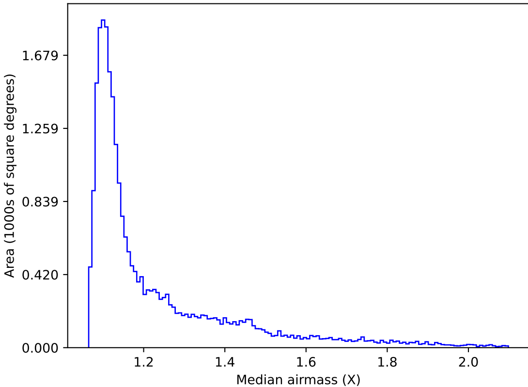
baseline_v3.2_10yrs Yr 1 all bands: Median airmass
