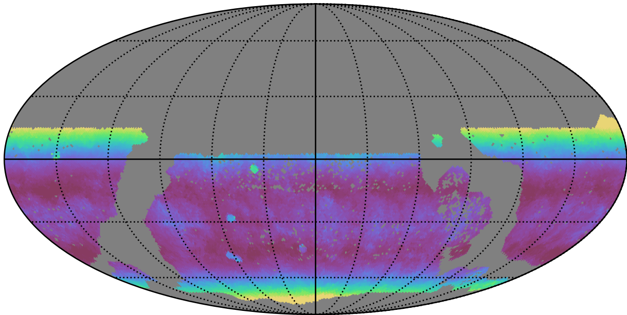
baseline_v3.2_10yrs WFD z band: Median airmass
