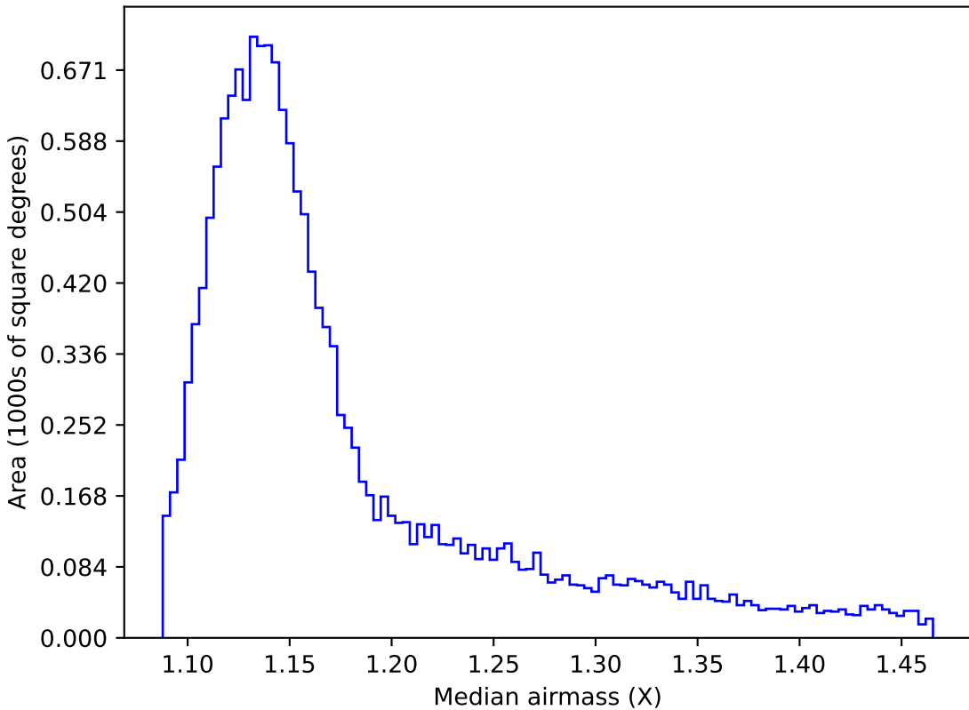
baseline_v3.2_10yrs WFD z band: Median airmass
