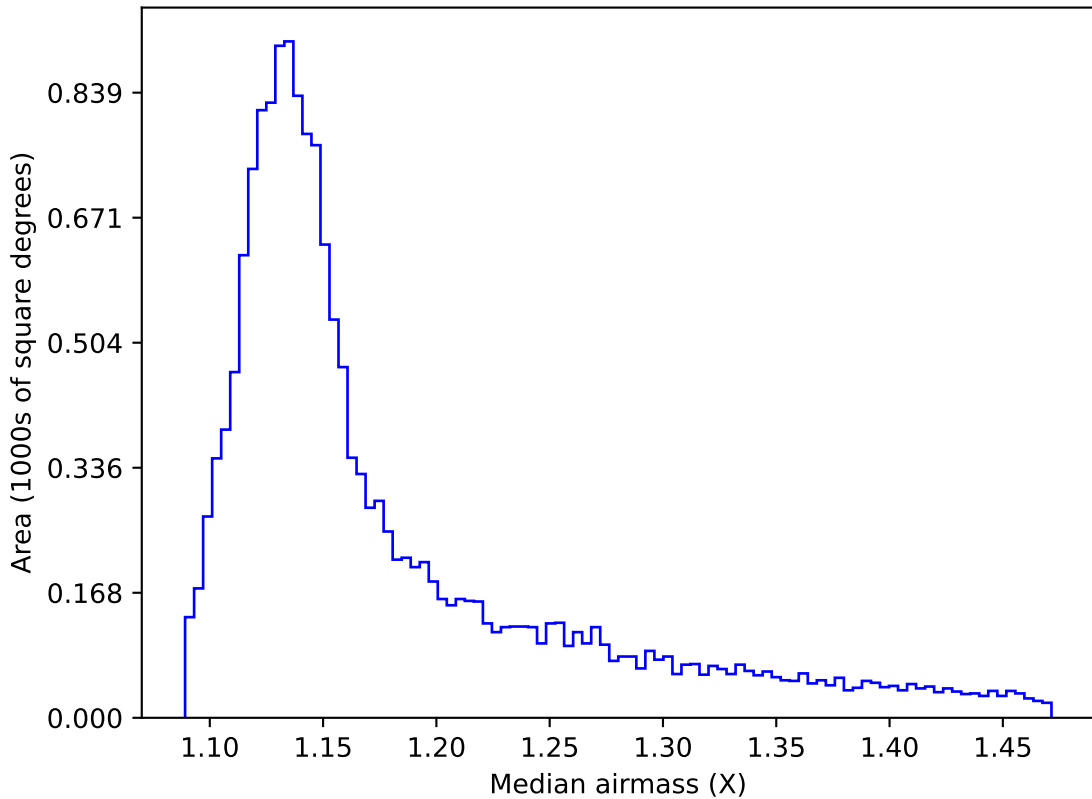
baseline_v3.2_10yrs WFD y band: Median airmass
