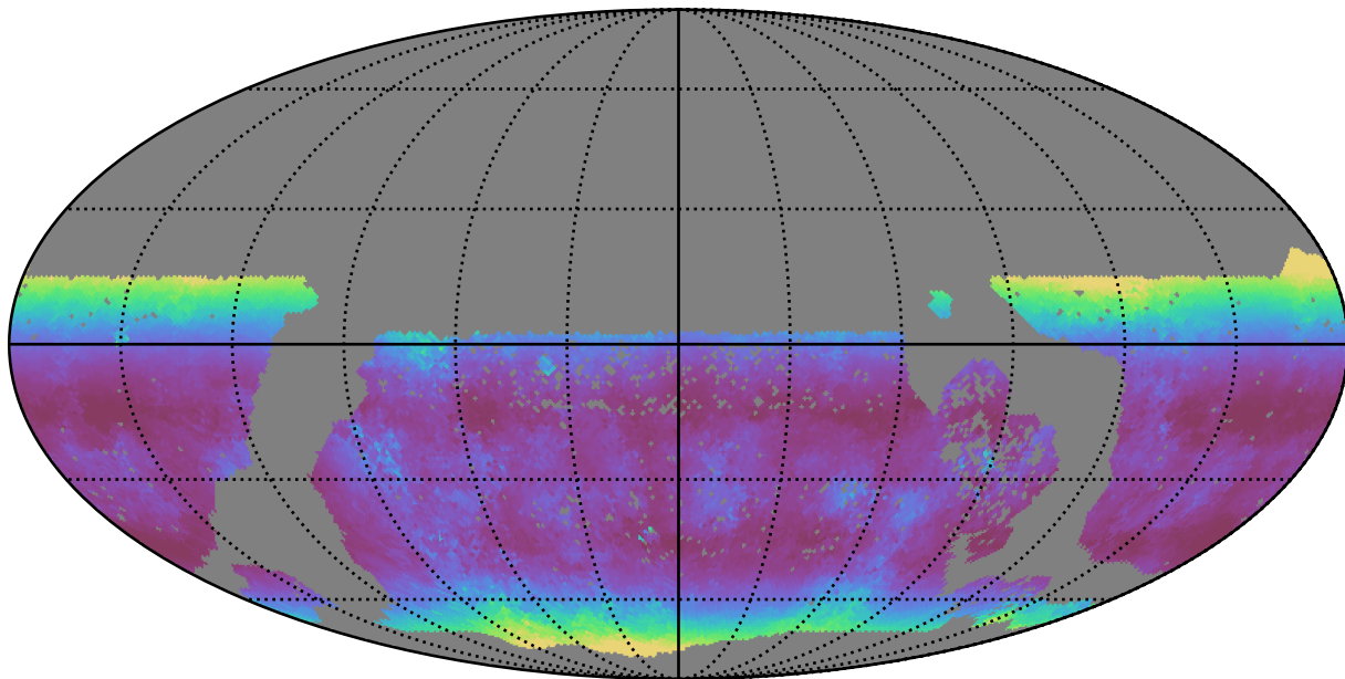
baseline_v3.2_10yrs WFD u band: Median airmass
