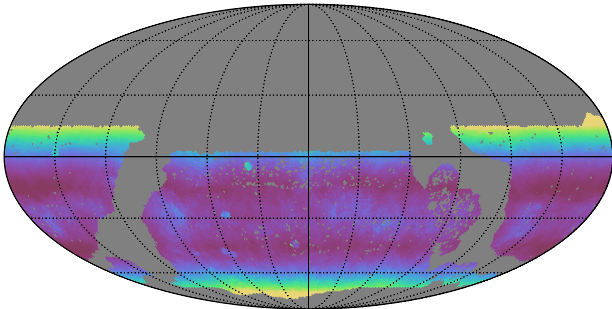
baseline_v3.2_10yrs WFD r band: Median airmass
