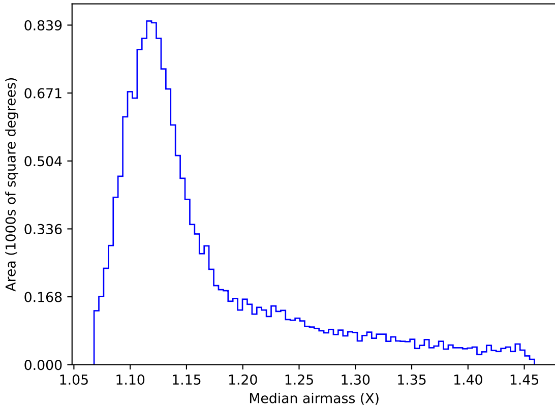
baseline_v3.2_10yrs WFD r band: Median airmass
