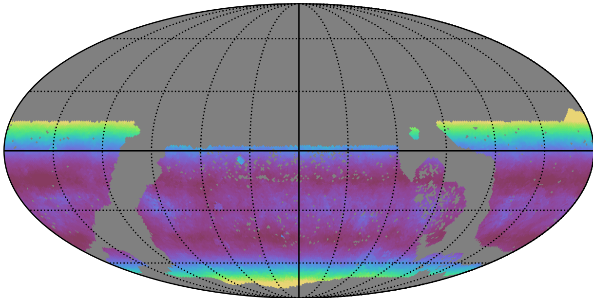
baseline_v3.2_10yrs WFD i band: Median airmass
