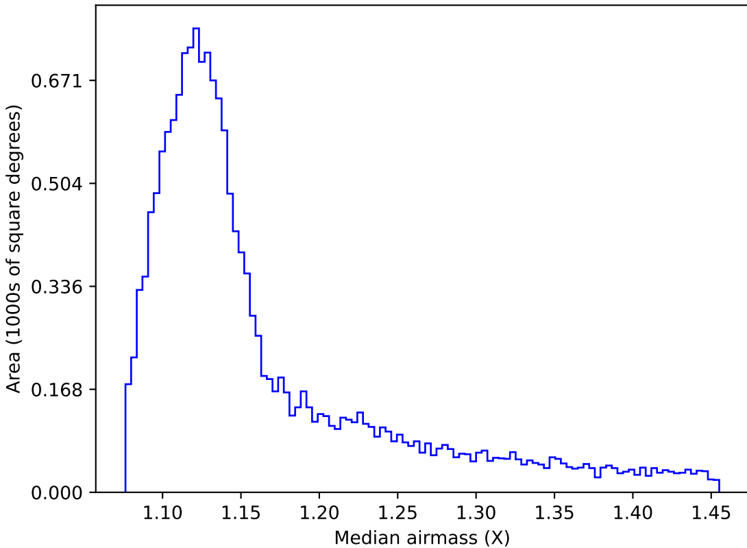
baseline_v3.2_10yrs WFD i band: Median airmass
