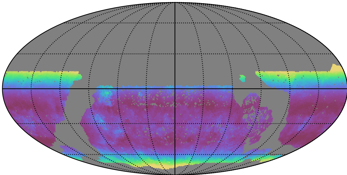
baseline_v3.2_10yrs WFD g band: Median airmass
