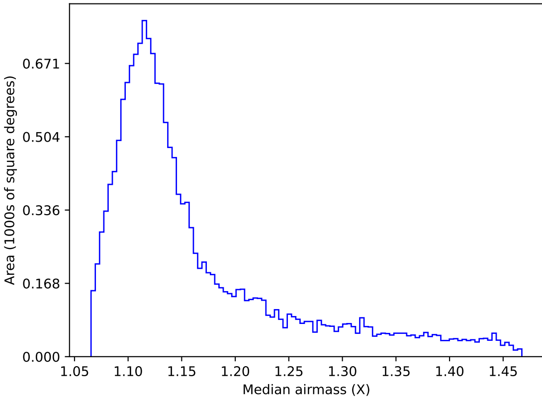
baseline_v3.2_10yrs WFD g band: Median airmass
