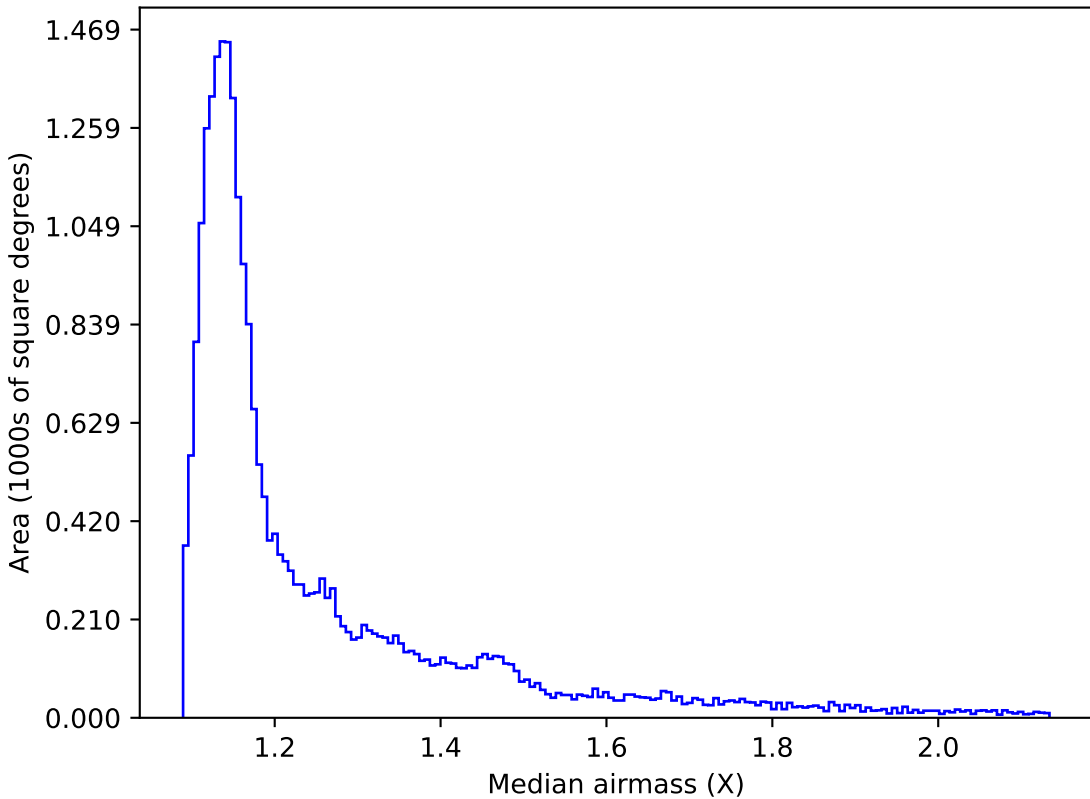
baseline_v3.2_10yrs All sky z band: Median airmass
