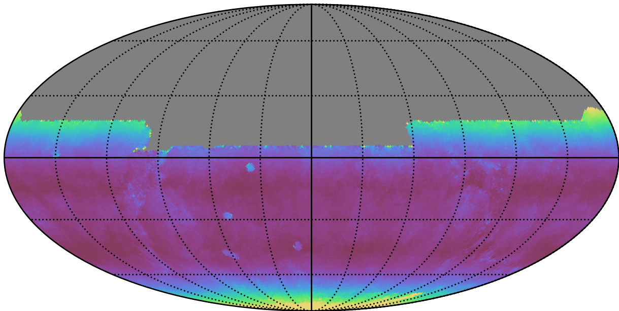
baseline_v3.2_10yrs All sky y band: Median airmass
