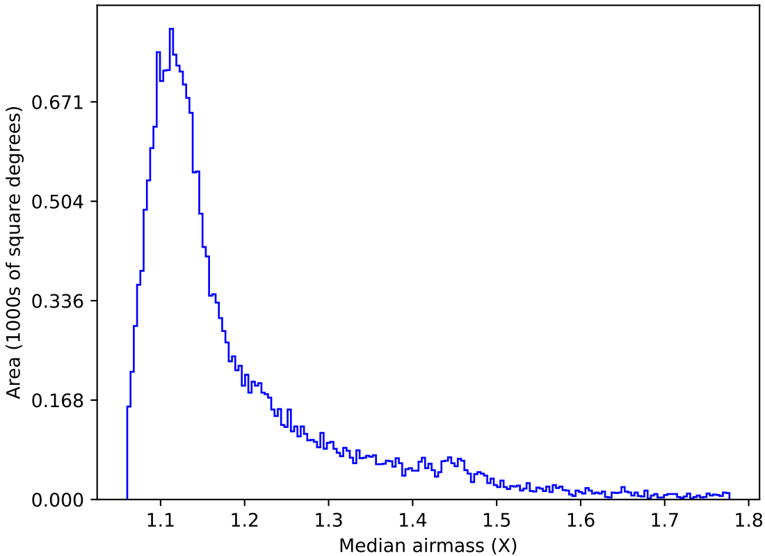
baseline_v3.2_10yrs All sky u band: Median airmass
