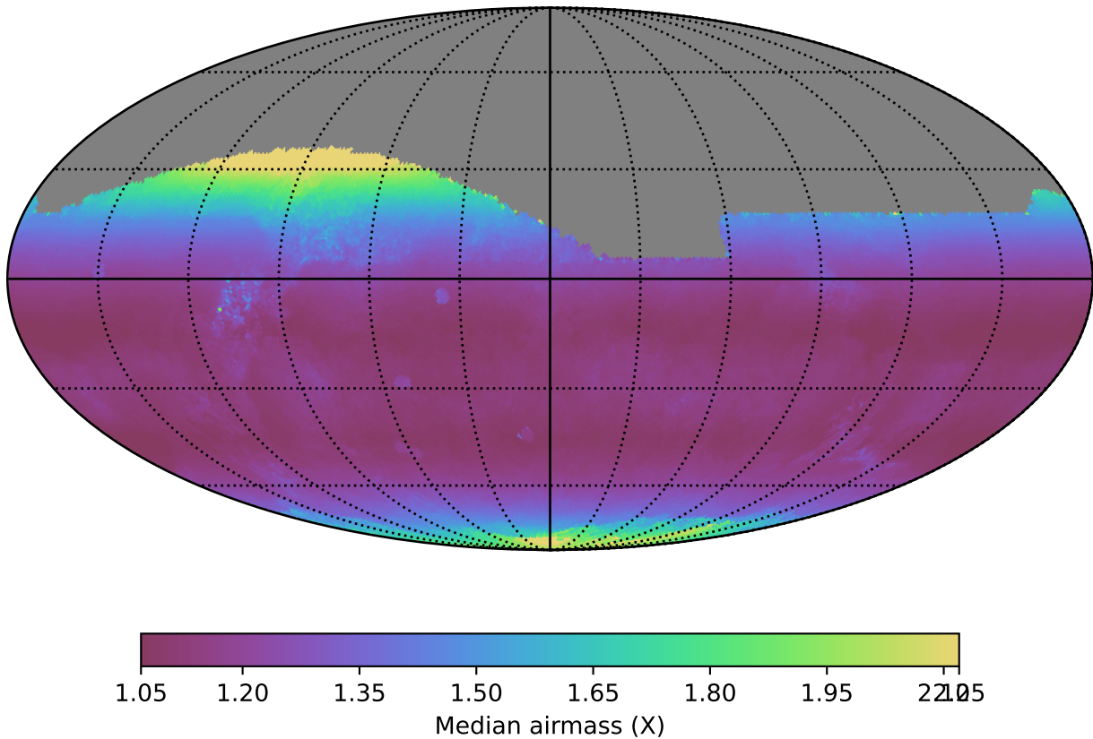
baseline_v3.2_10yrs All sky r band: Median airmass
