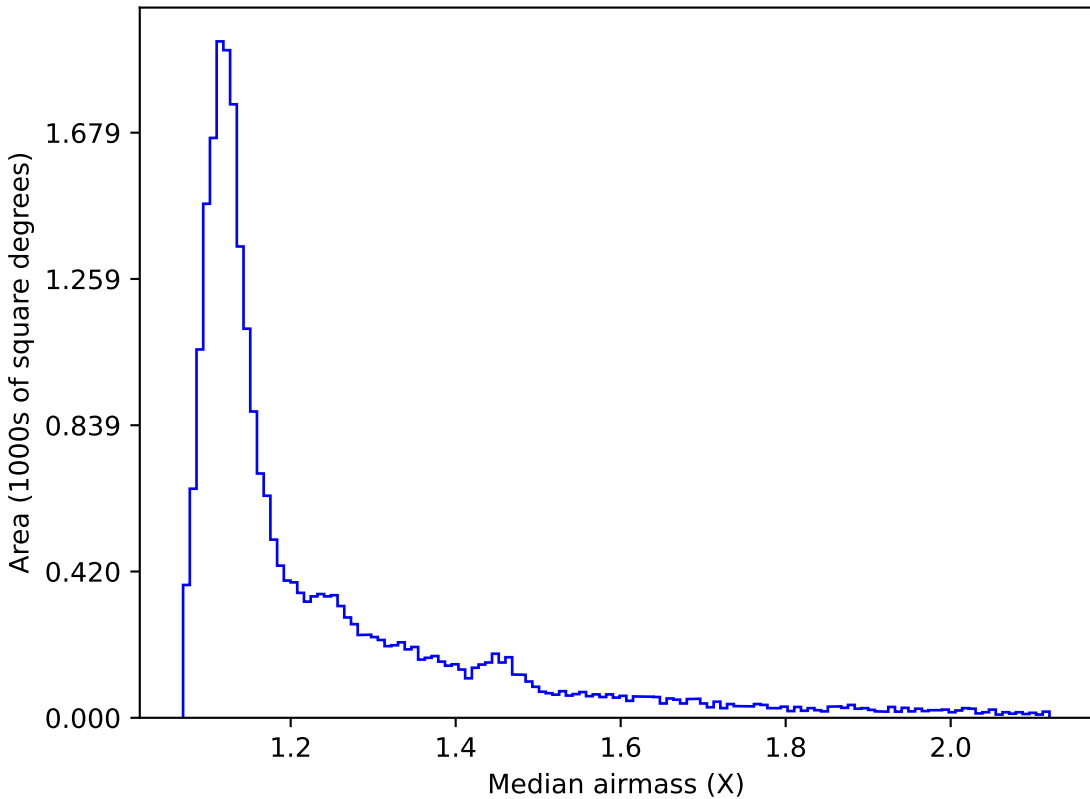
baseline_v3.2_10yrs All sky r band: Median airmass
