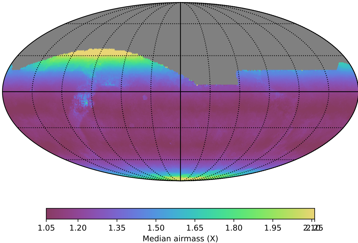
baseline_v3.2_10yrs All sky i band: Median airmass
