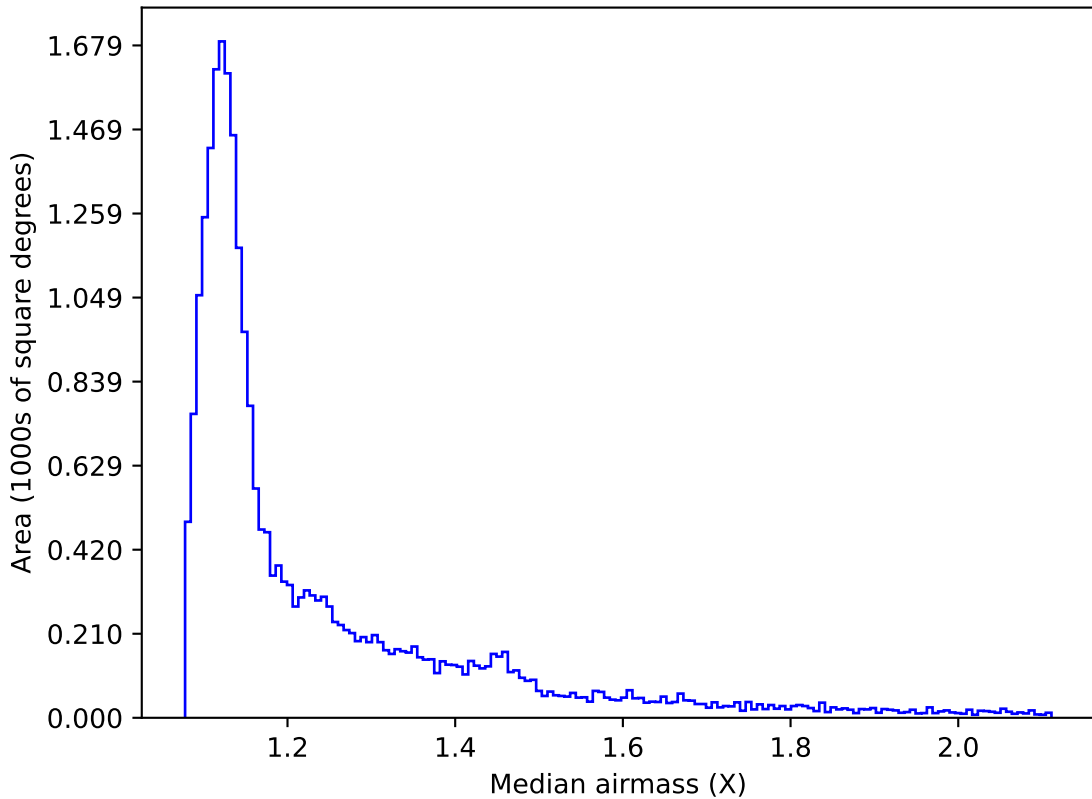
baseline_v3.2_10yrs All sky i band: Median airmass
