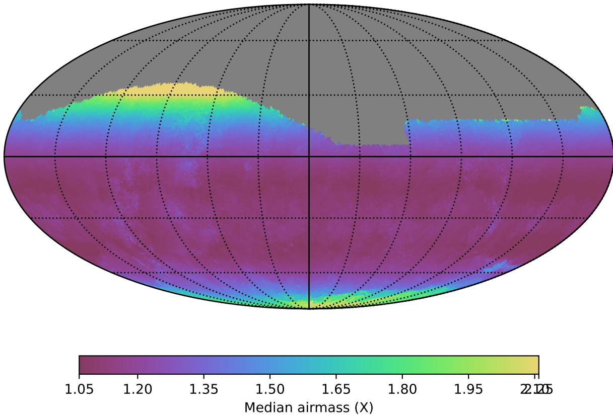
baseline_v3.2_10yrs All sky g band: Median airmass
