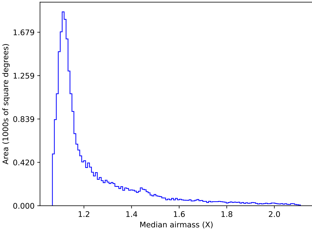
baseline_v3.2_10yrs All sky g band: Median airmass
