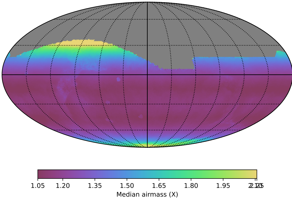
baseline_v3.2_10yrs All sky all bands: Median airmass
