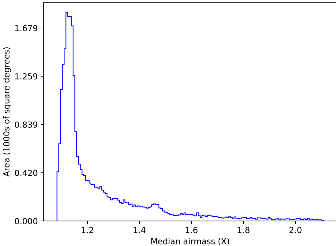
baseline_v3.2_10yrs All sky all bands: Median airmass
