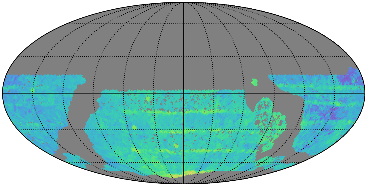
baseline_v3.2_10yrs WFD z band: Median Season Length
