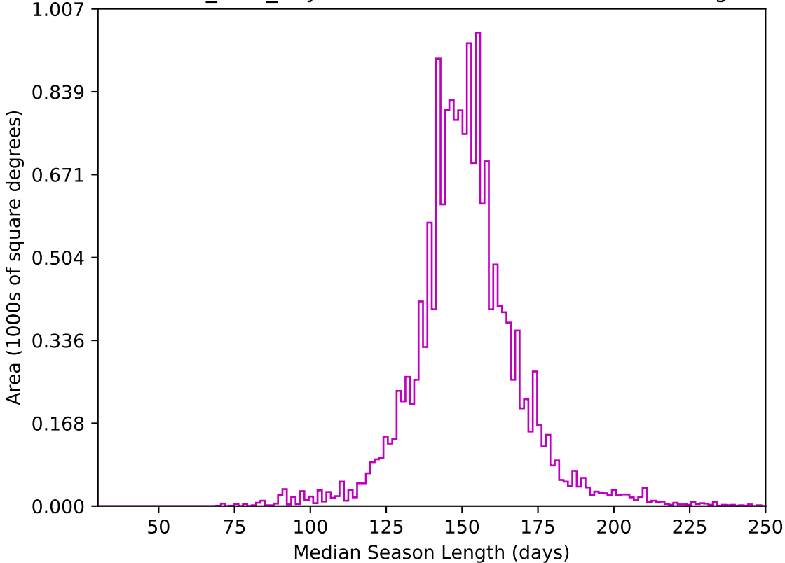
baseline_v3.2_10yrs WFD z band: Median Season Length
