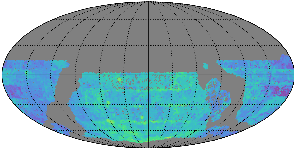
baseline_v3.2_10yrs WFD y band: Median Season Length
