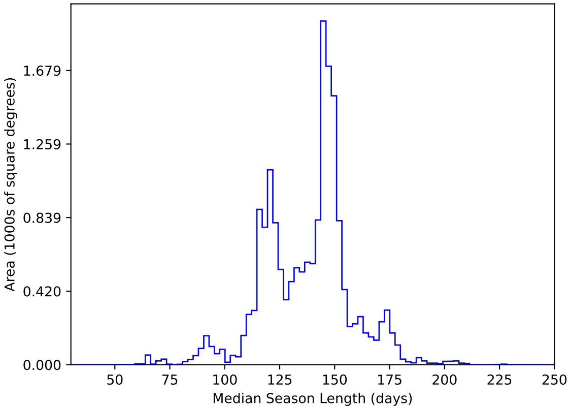
baseline_v3.2_10yrs WFD y band: Median Season Length
