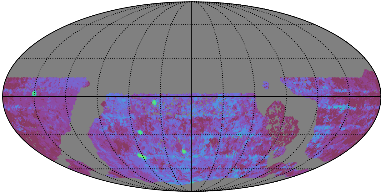
baseline_v3.2_10yrs WFD u band: Median Season Length
