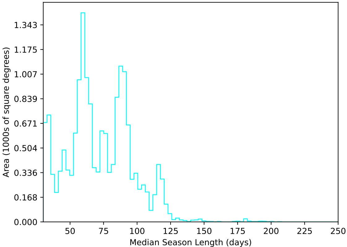
baseline_v3.2_10yrs WFD u band: Median Season Length
